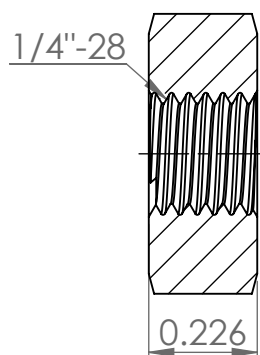
SIDE (BREAKOUT)
