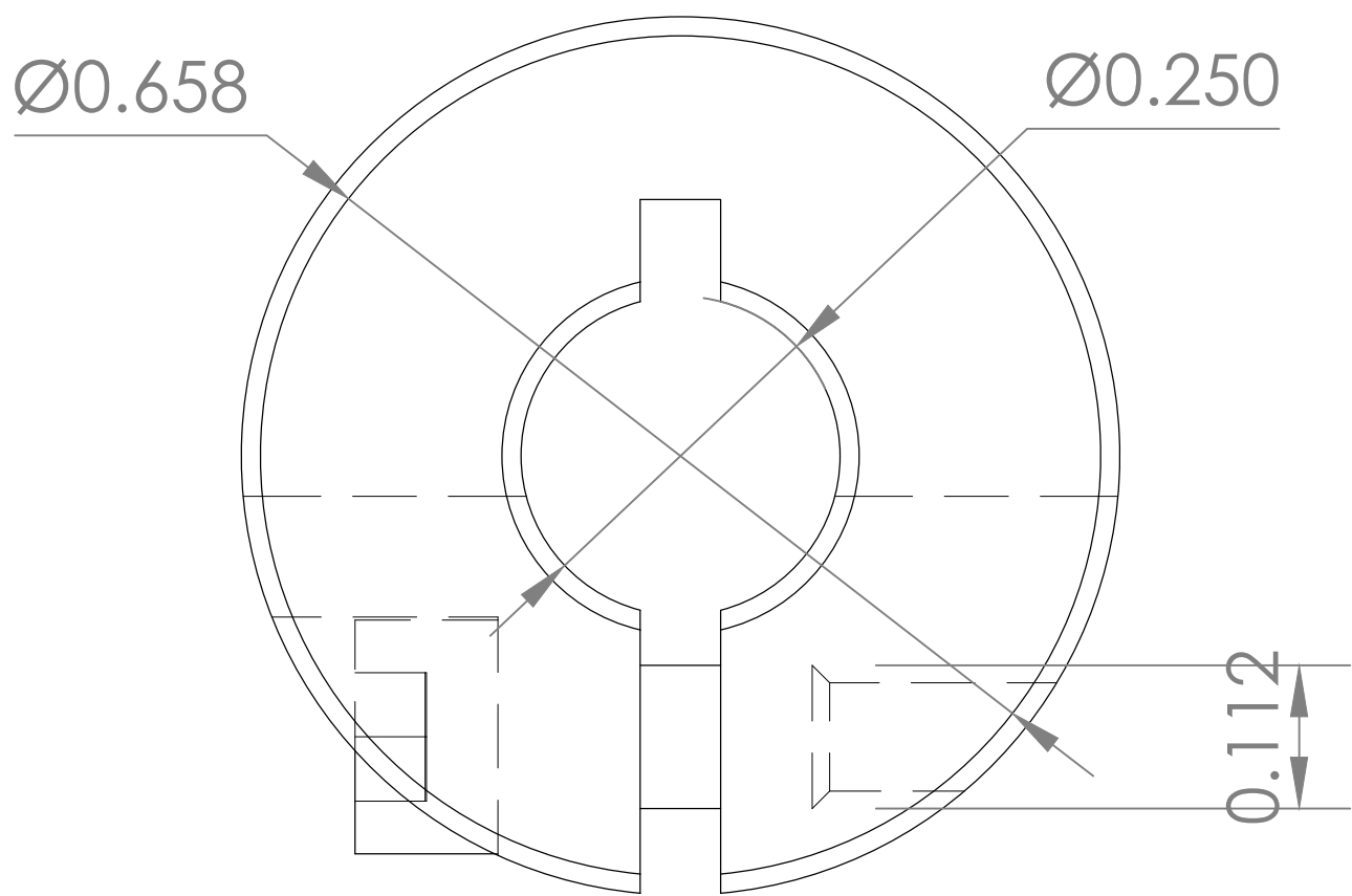
SIDE
