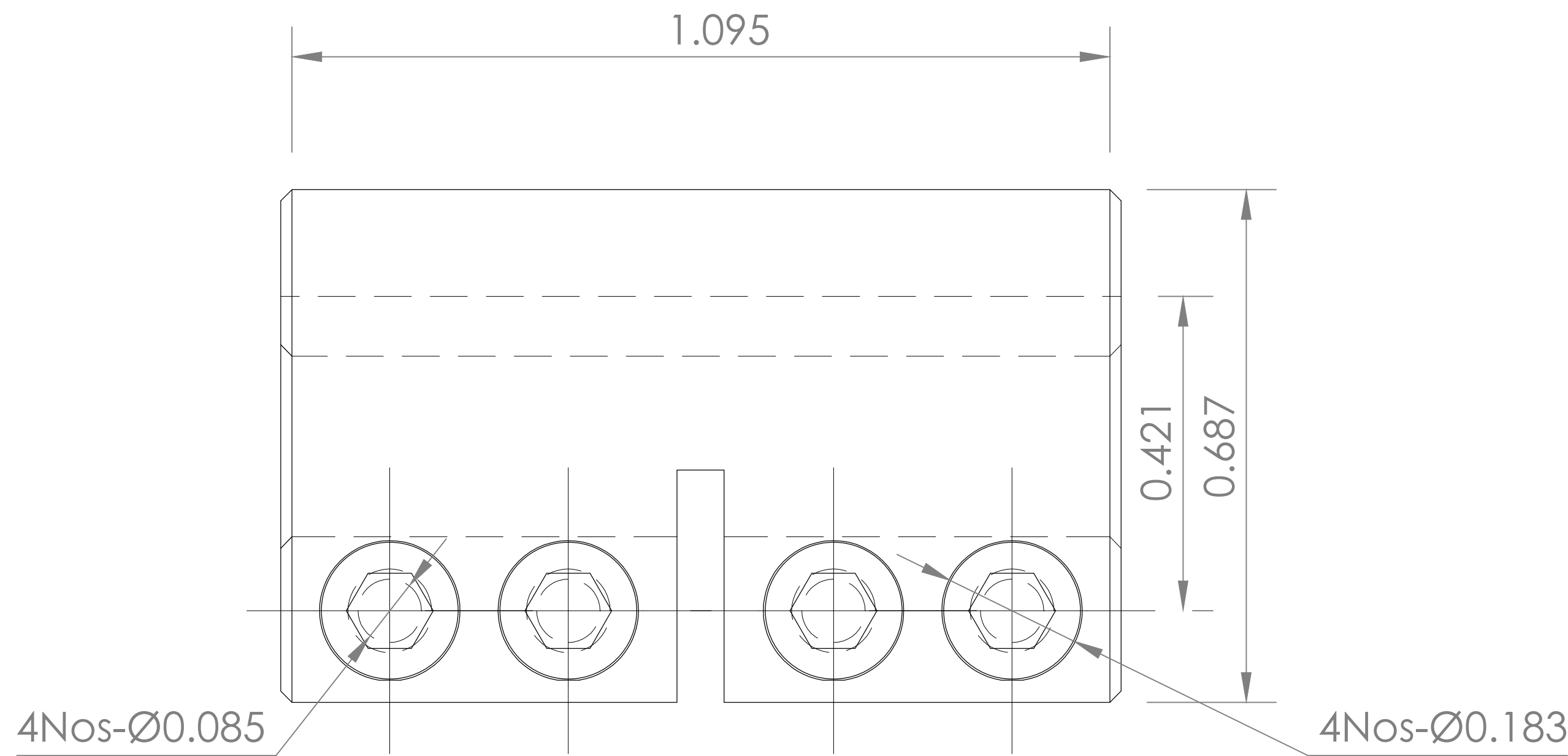
FRONT
