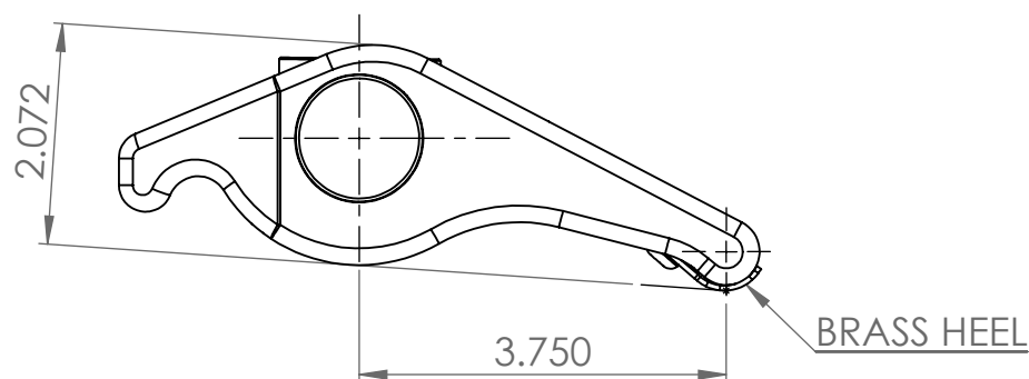
FRONT
