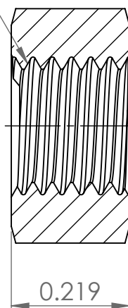
SIDE (BREAKOUT)
