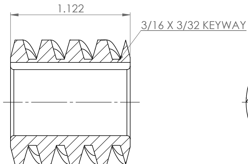
SIDE (BREAKOUT)
