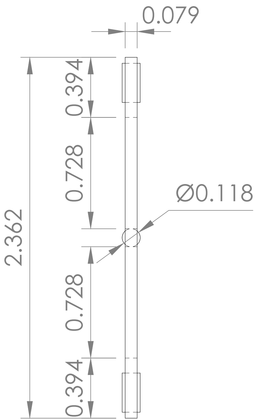
FRONT
