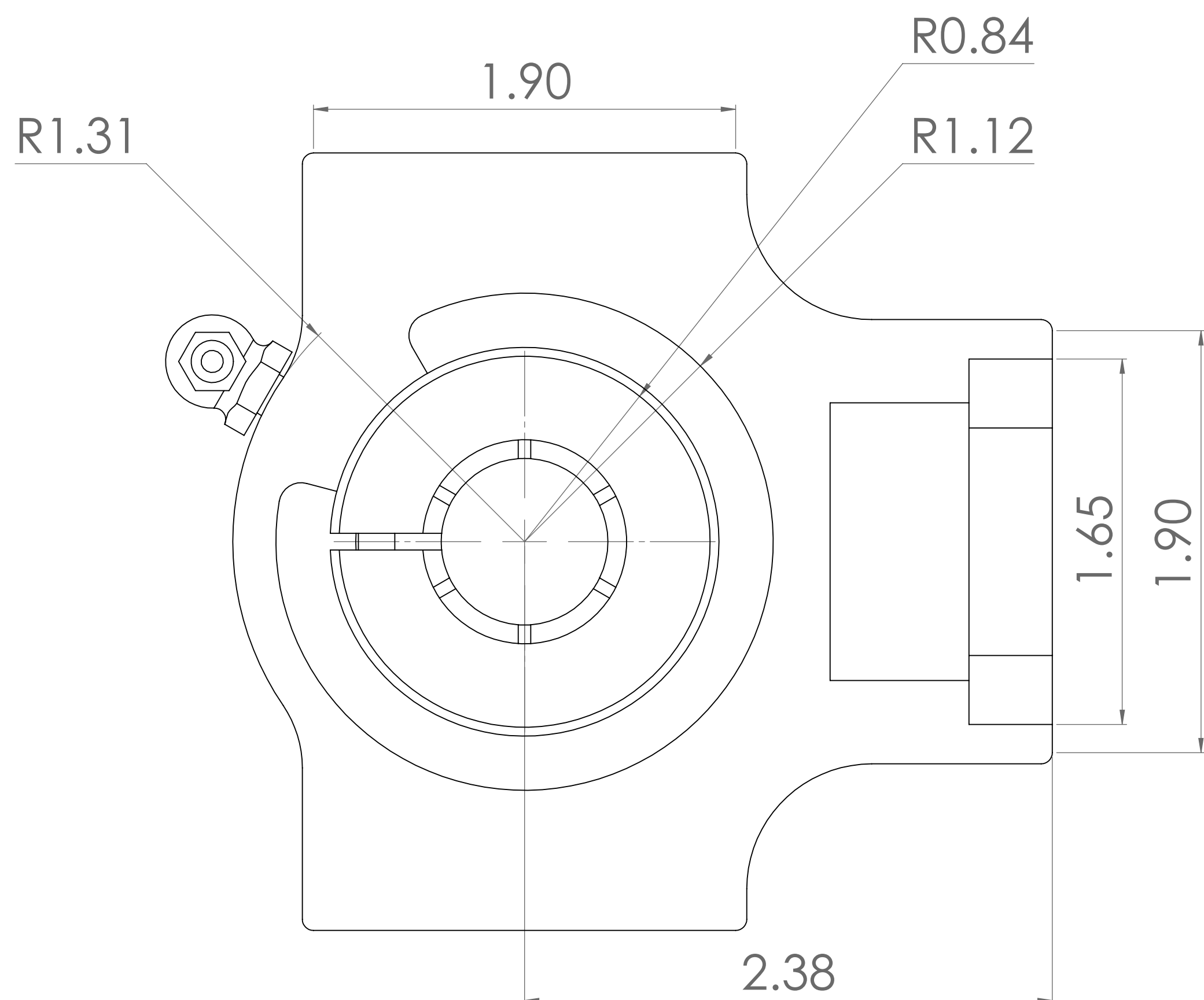
FRONT
